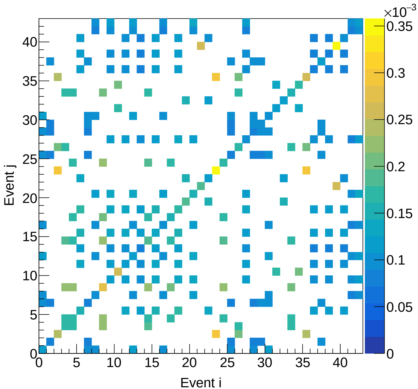
LH2 (total) Covariance | M: [4.2, 4.5] xF: [0.80, 0.85)
