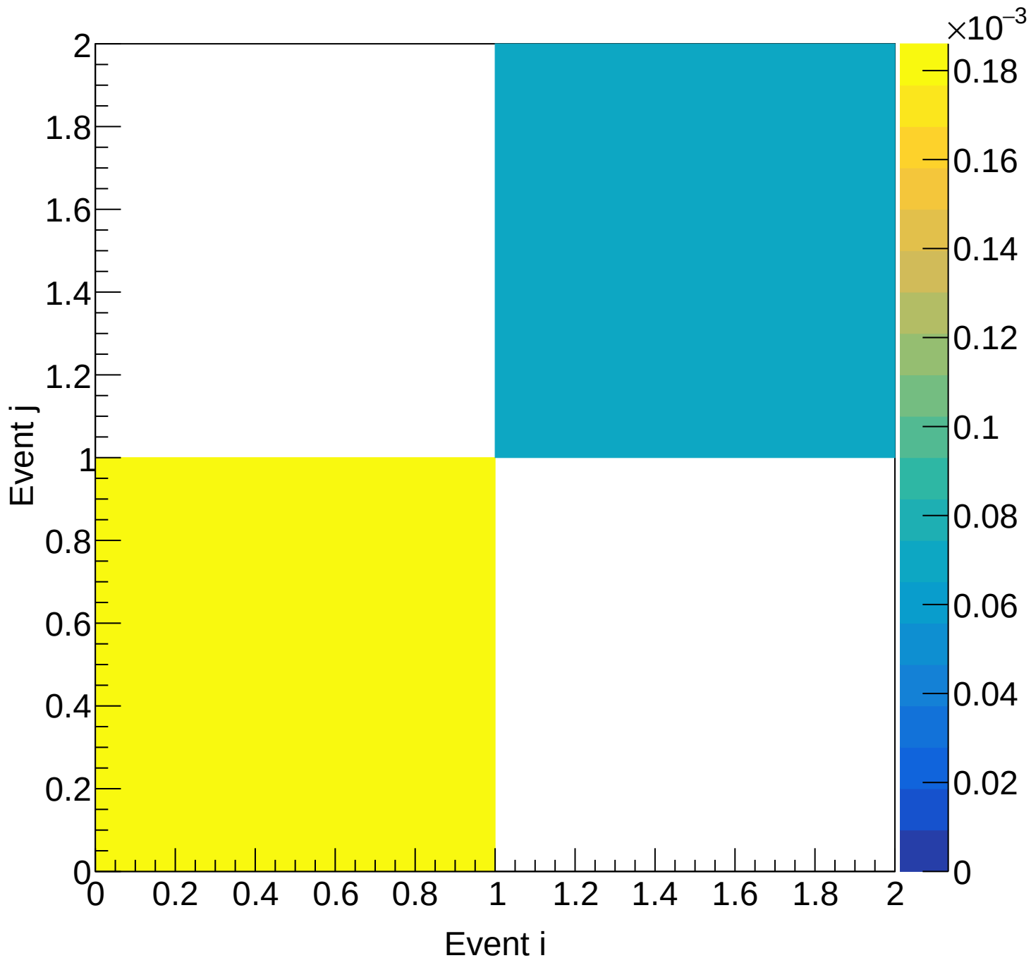
LH2 (total) Covariance | M: [6.9, 7.5] xF: [0.80, 0.85]
