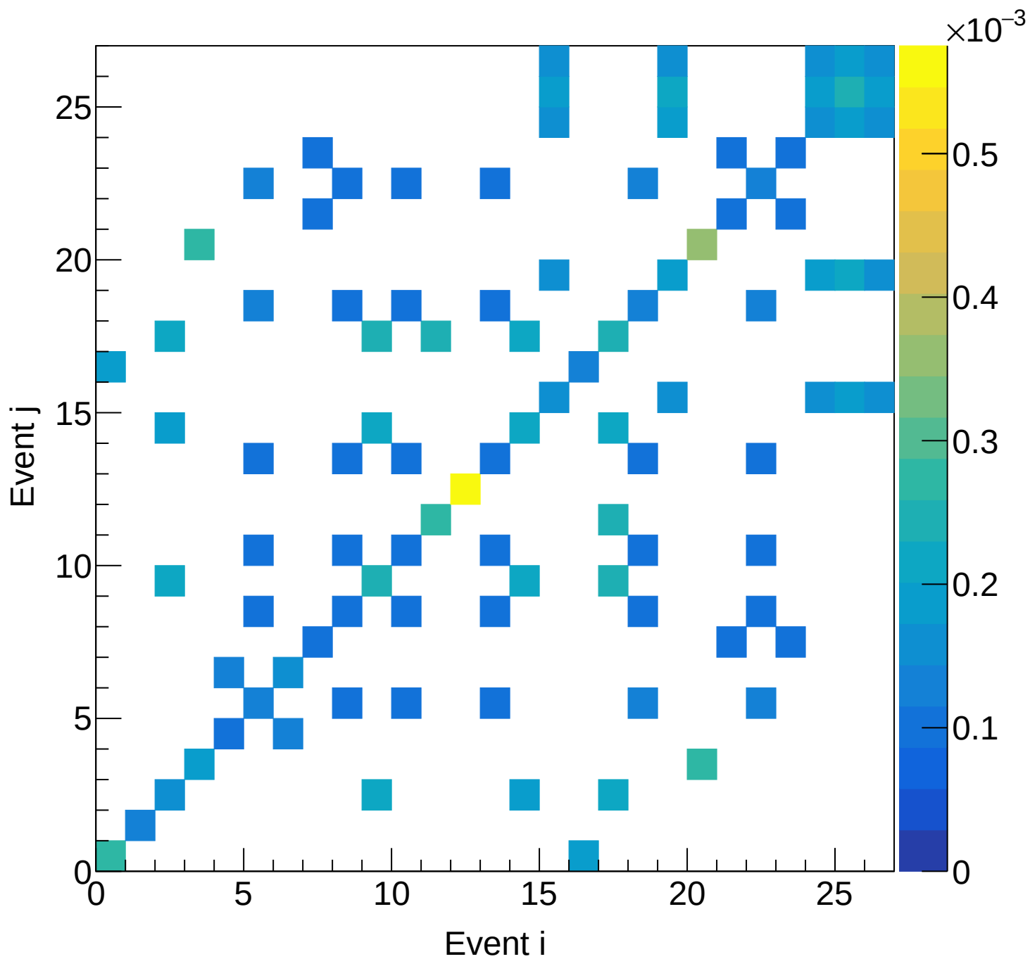
LH2 (total) Covariance | M: [4.5, 4.8) xF: [0.80, 0.85)
