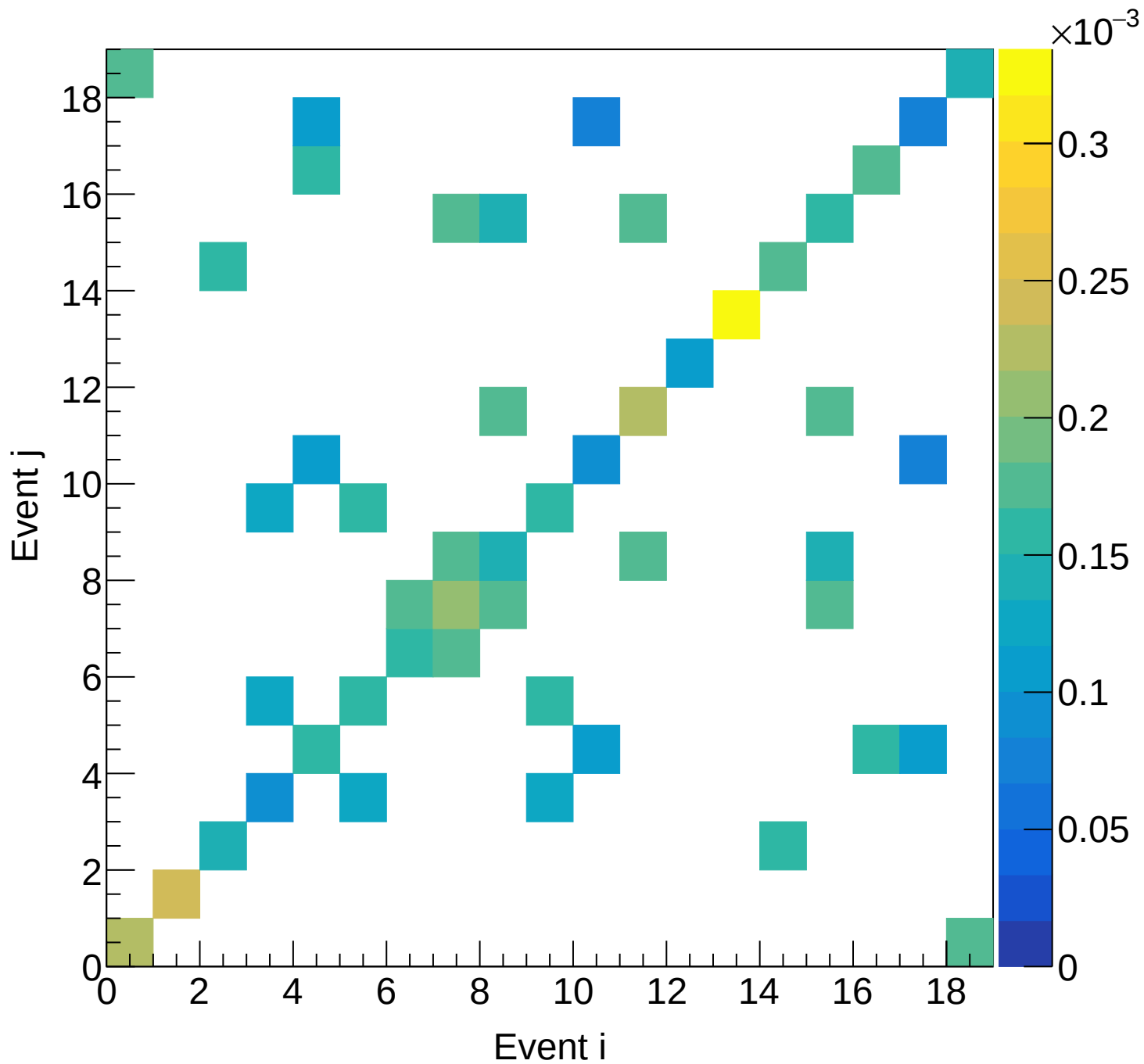
LH2 (total) Covariance | M: [4.8, 5.1) xF: [0.80, 0.85)
