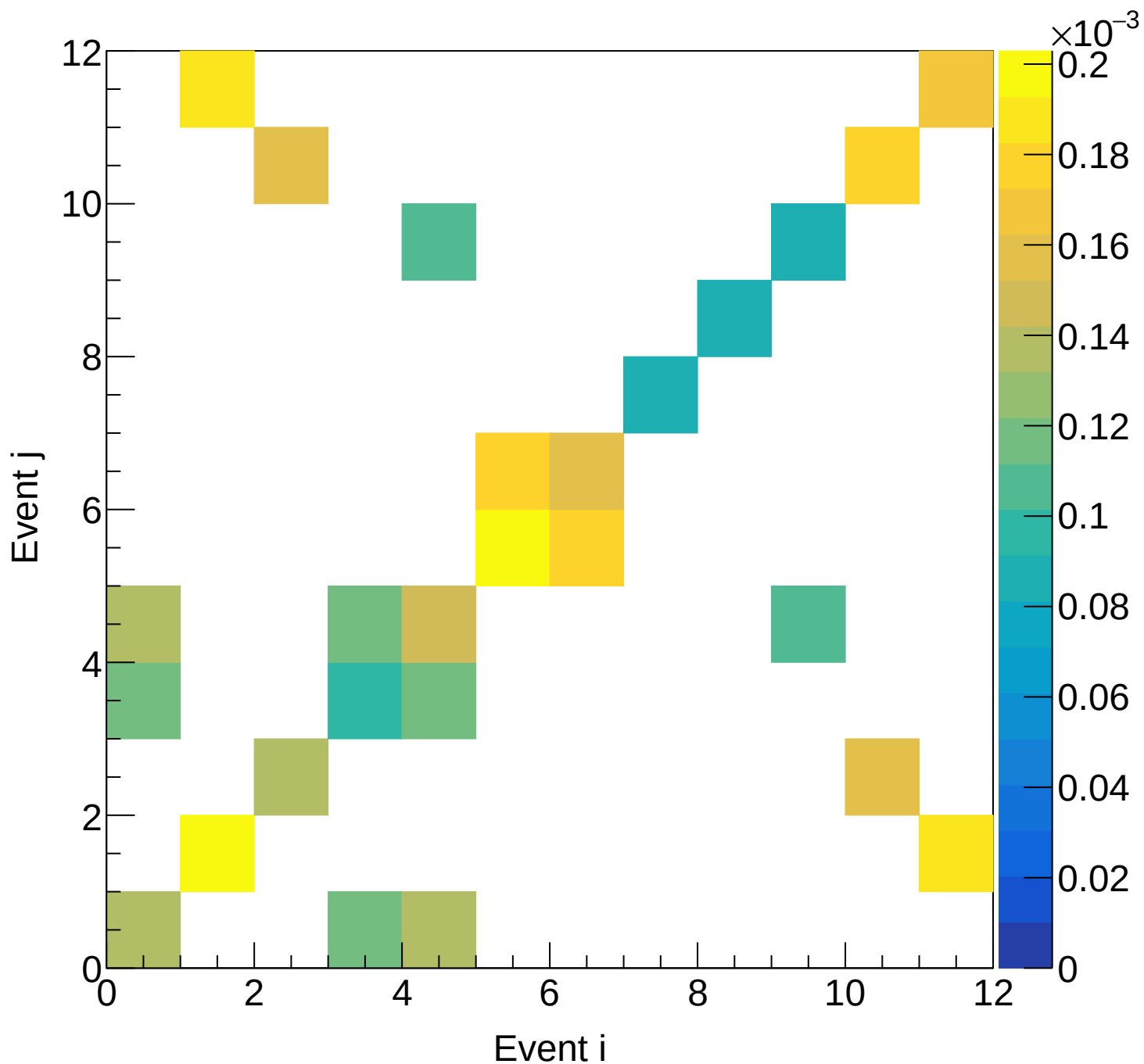
LH2 (total) Covariance | M: [5.1, 5.4) xF: [0.80, 0.85)
