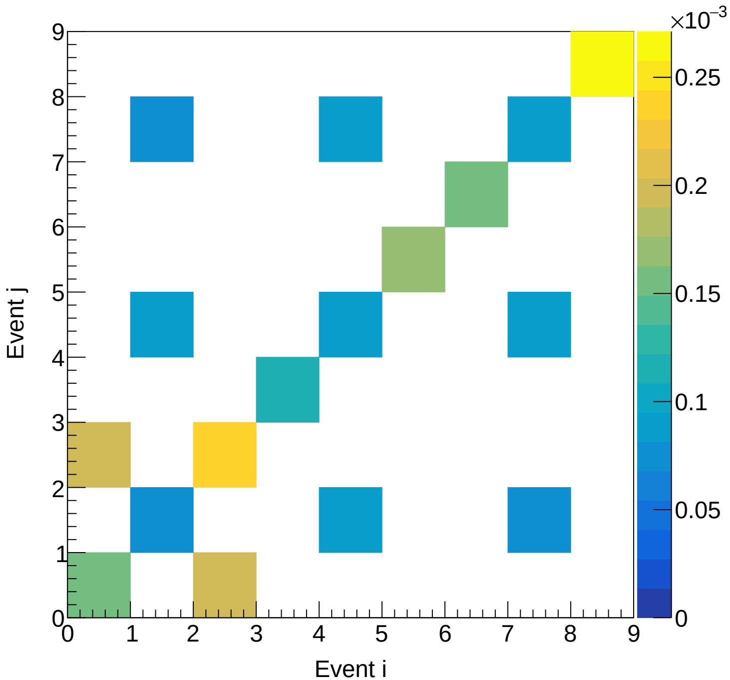
LH2 (total) Covariance | M: [5.4, 5.7) xF: [0.80, 0.85)
