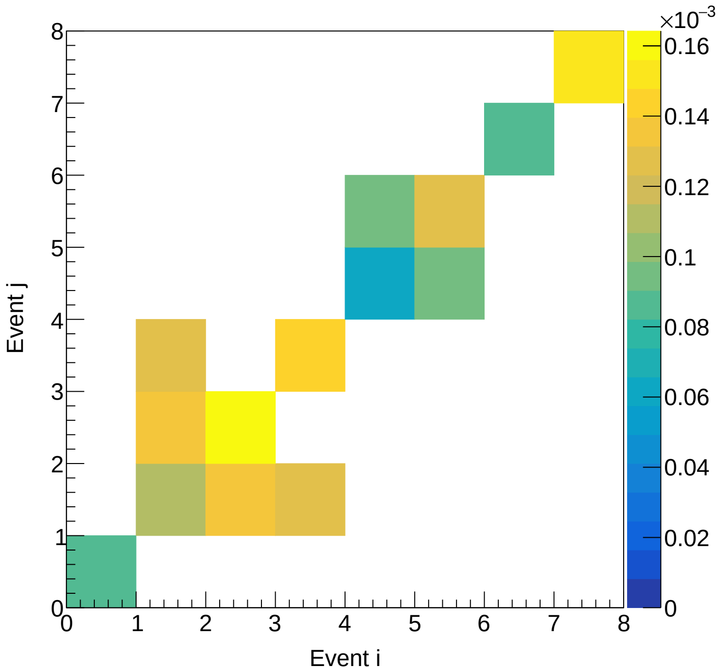
LH2 (total) Covariance | M: [5.7, 6.0] xF: [0.80, 0.85)
