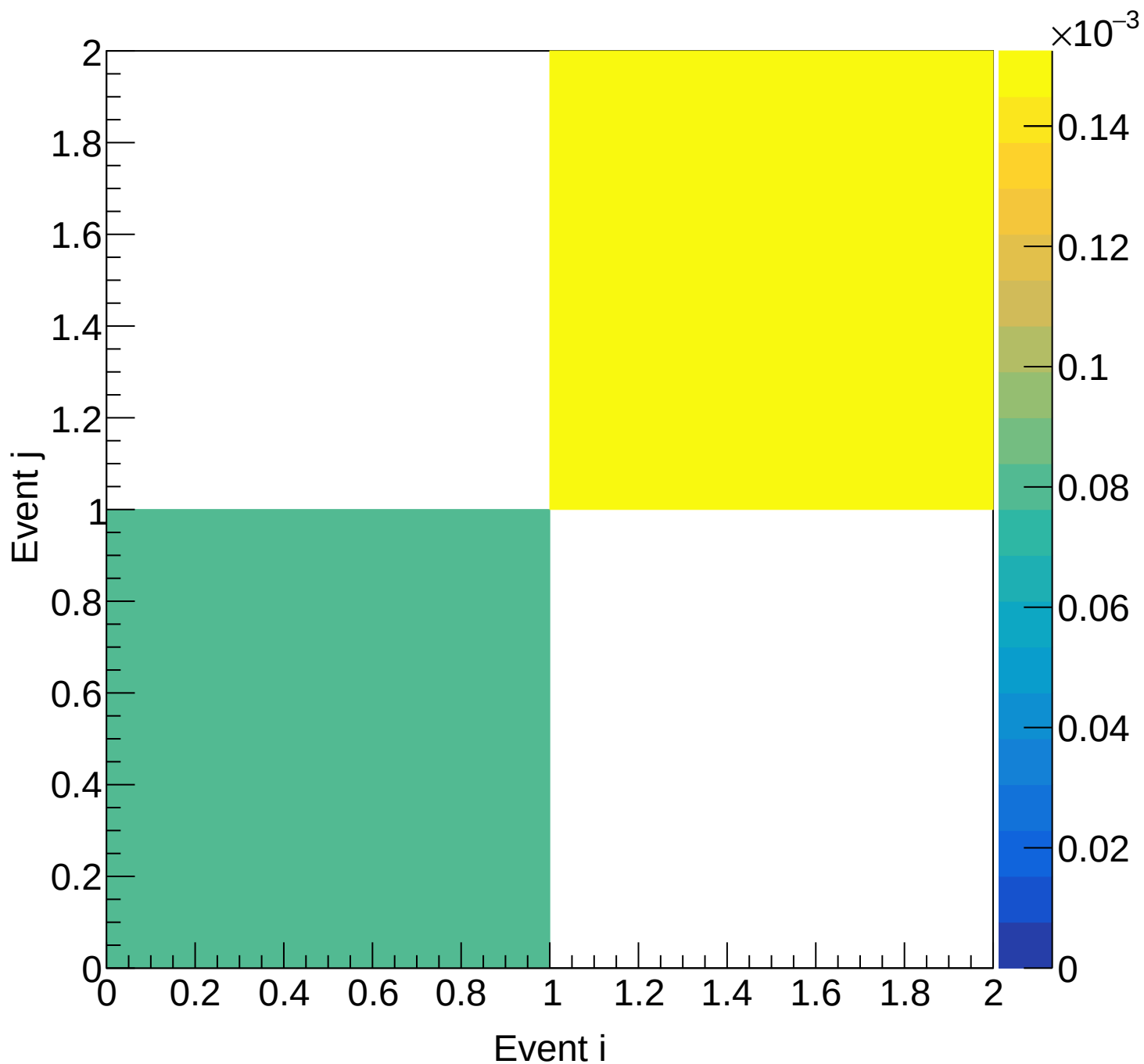
LH2 (total) Covariance | M: [6.6, 6.9) xF: [0.80, 0.85)
