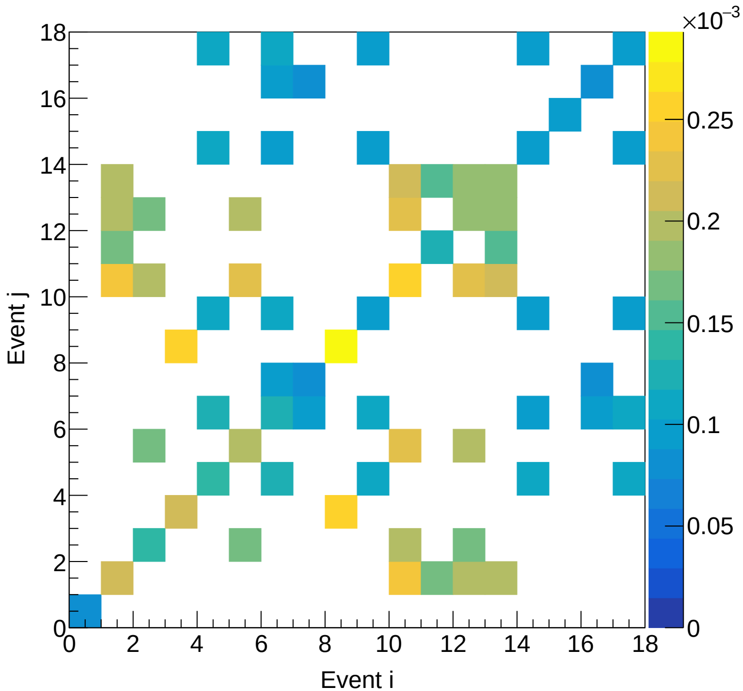
LH2 (total) Covariance | M: [4.2, 4.5) xF: [0.85, 0.90)
