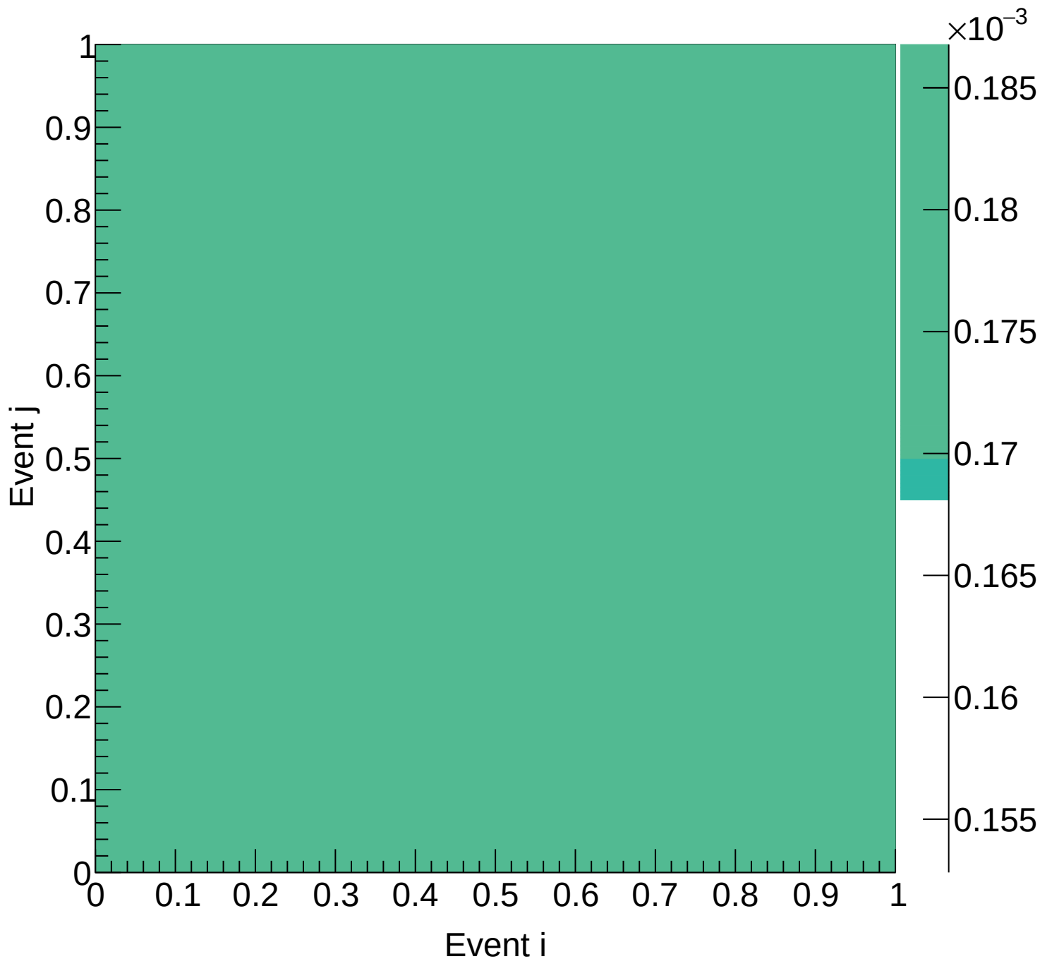
LH2 (total) Covariance | M: [6.9, 7.5] xF: [0.85, 0.90)
