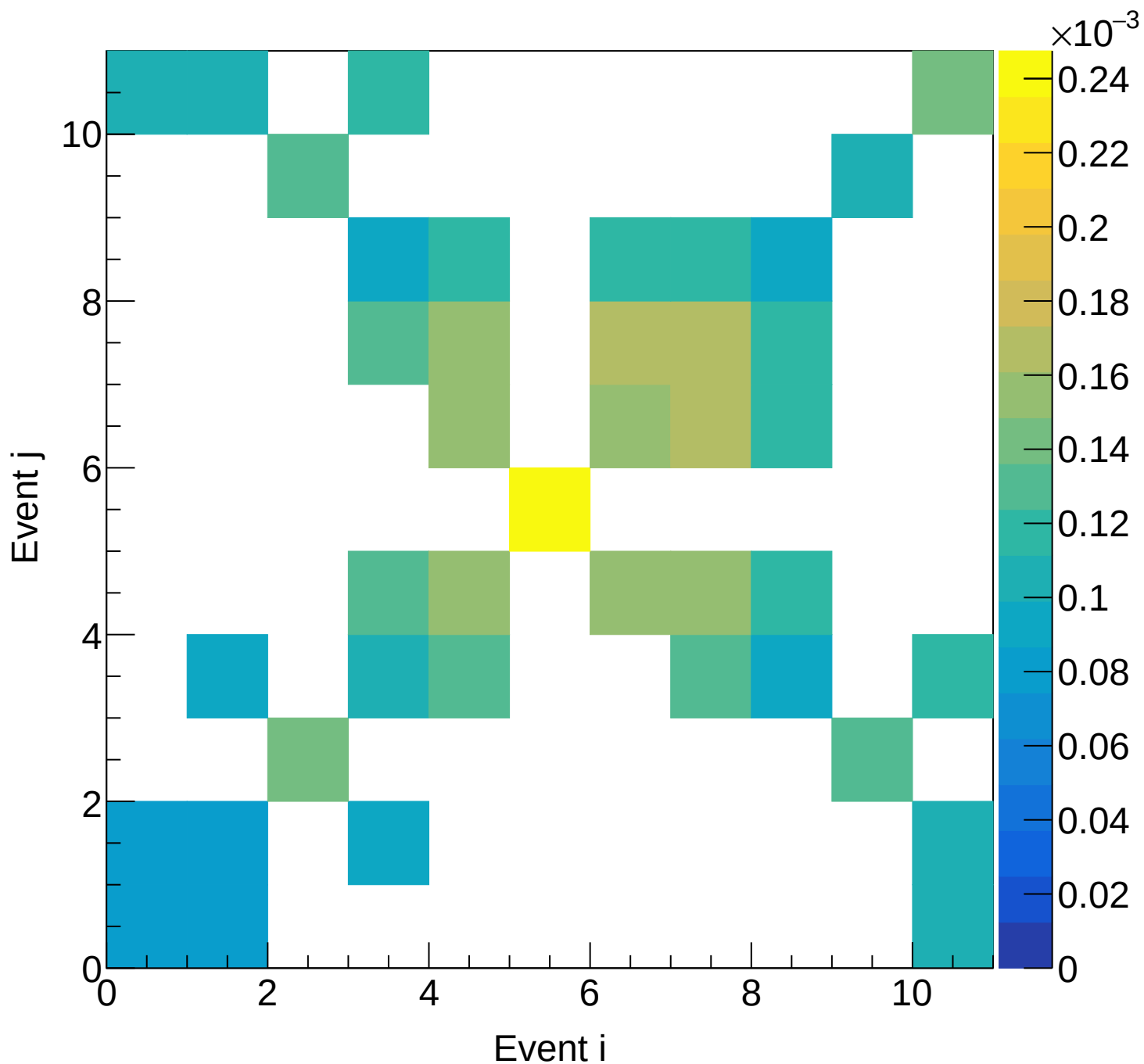
LH2 (total) Covariance | M: [4.8, 5.1) xF: [0.85, 0.90)
