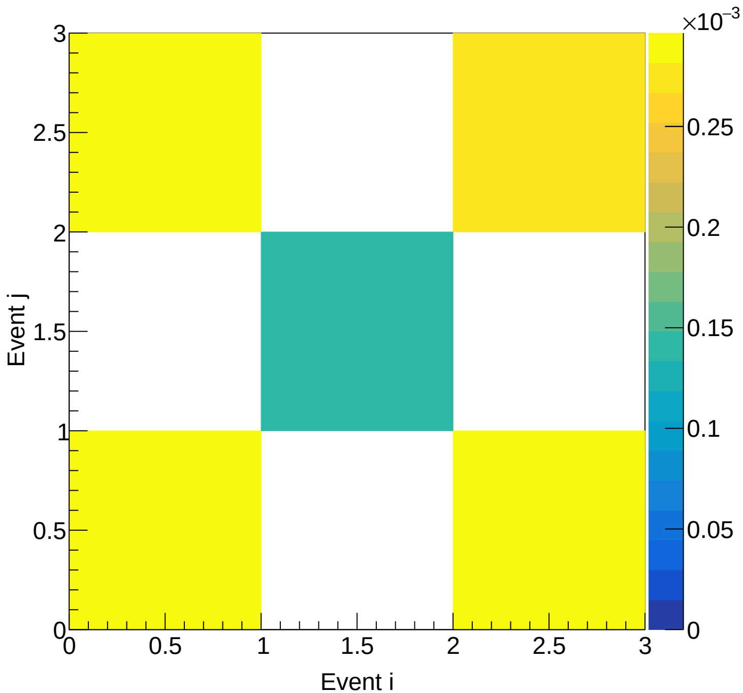
LH2 (total) Covariance | M: [5.4, 5.7) xF: [0.85, 0.90)
