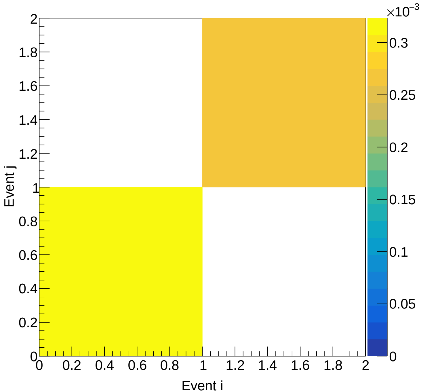
LH2 (total) Covariance | M: [6.6, 6.9) xF: [0.85, 0.90)
