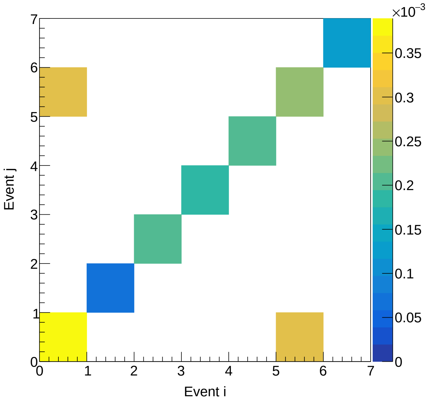
LH2 (total) Covariance | M: [3.9, 4.2) xF: [0.90, 0.95)
