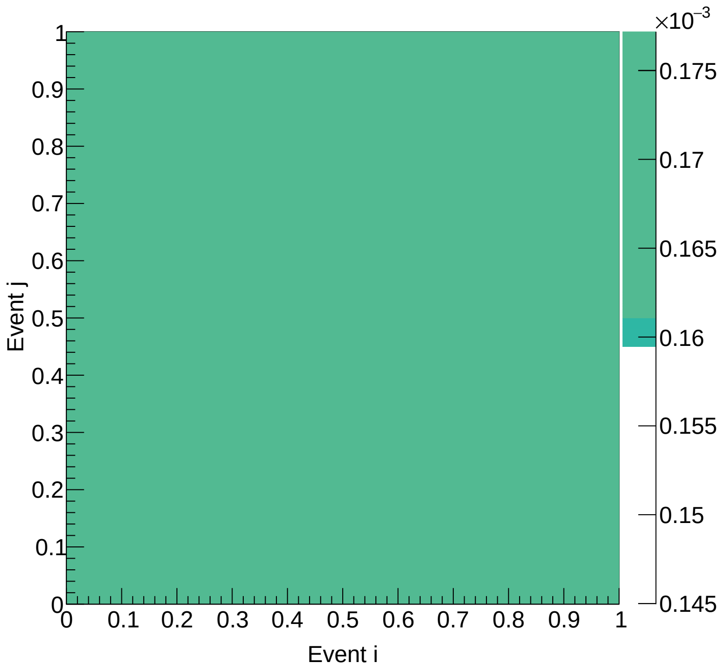
LH2 (total) Covariance | M: [4.8, 5.1) xF: [0.90, 0.95)
