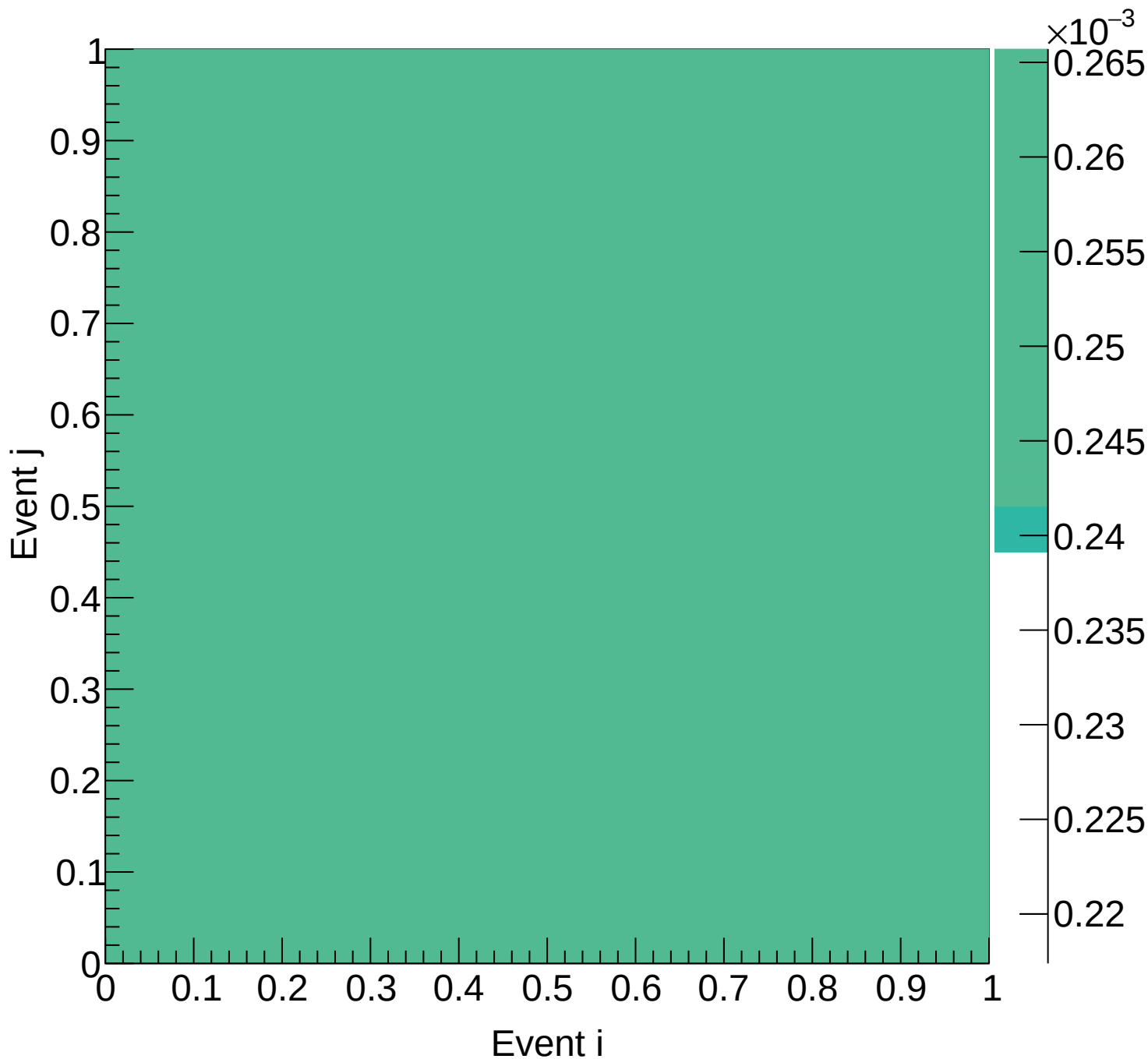
LH2 (total) Covariance | M: [5.4, 5.7) xF: [0.90, 0.95)
