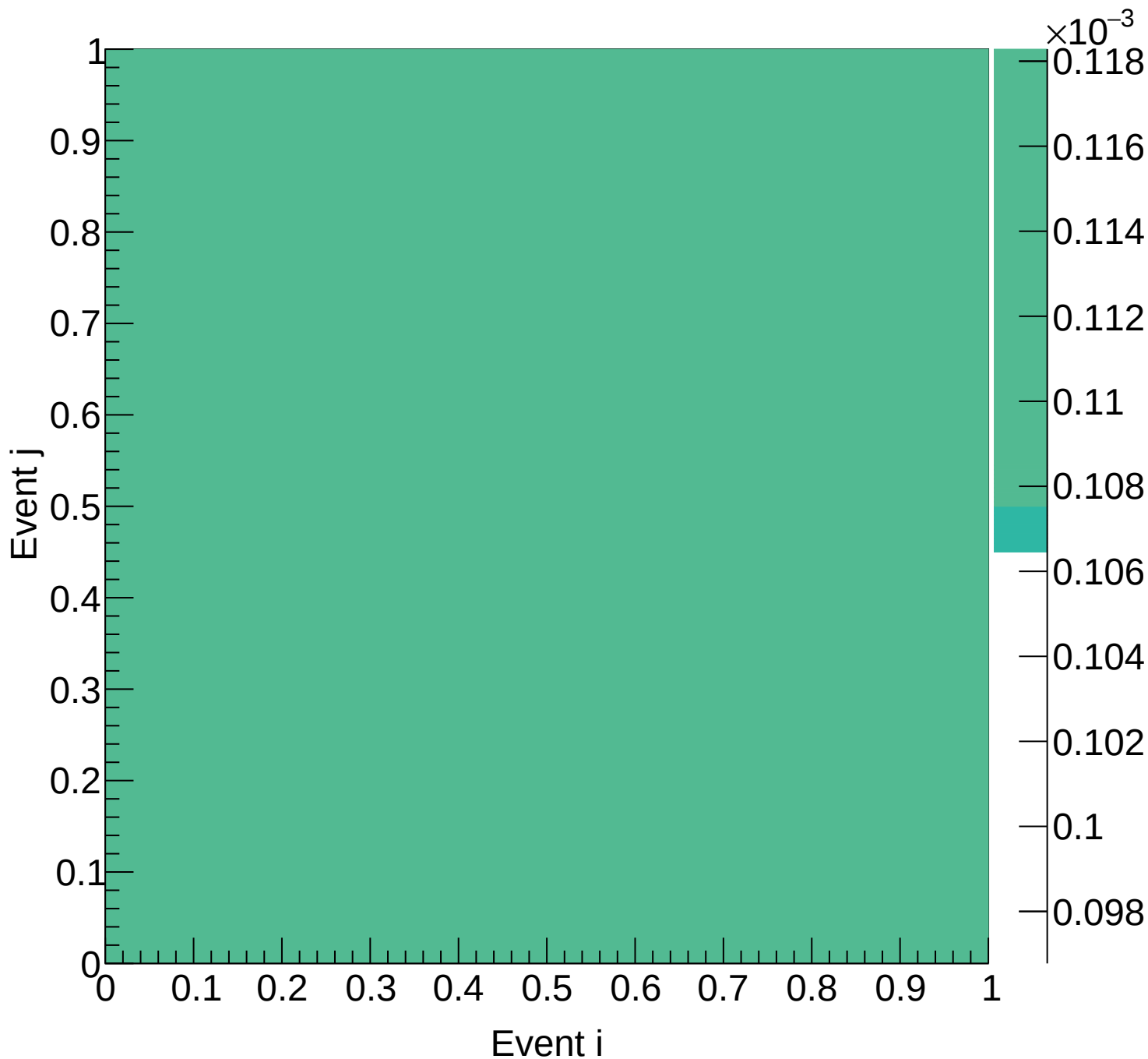
LH2 (total) Covariance | M: [7.5, 8.8) xF: [0.00, 0.05)
