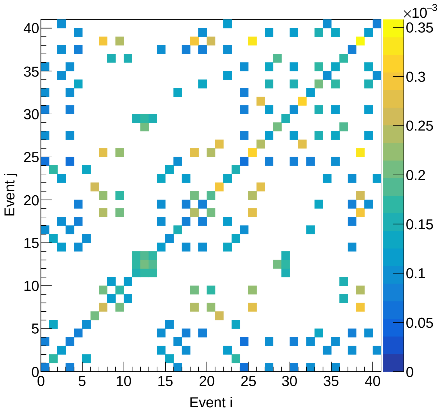
LH2 (total) Covariance | M: [4.8, 5.1) xF: [0.00, 0.05)
