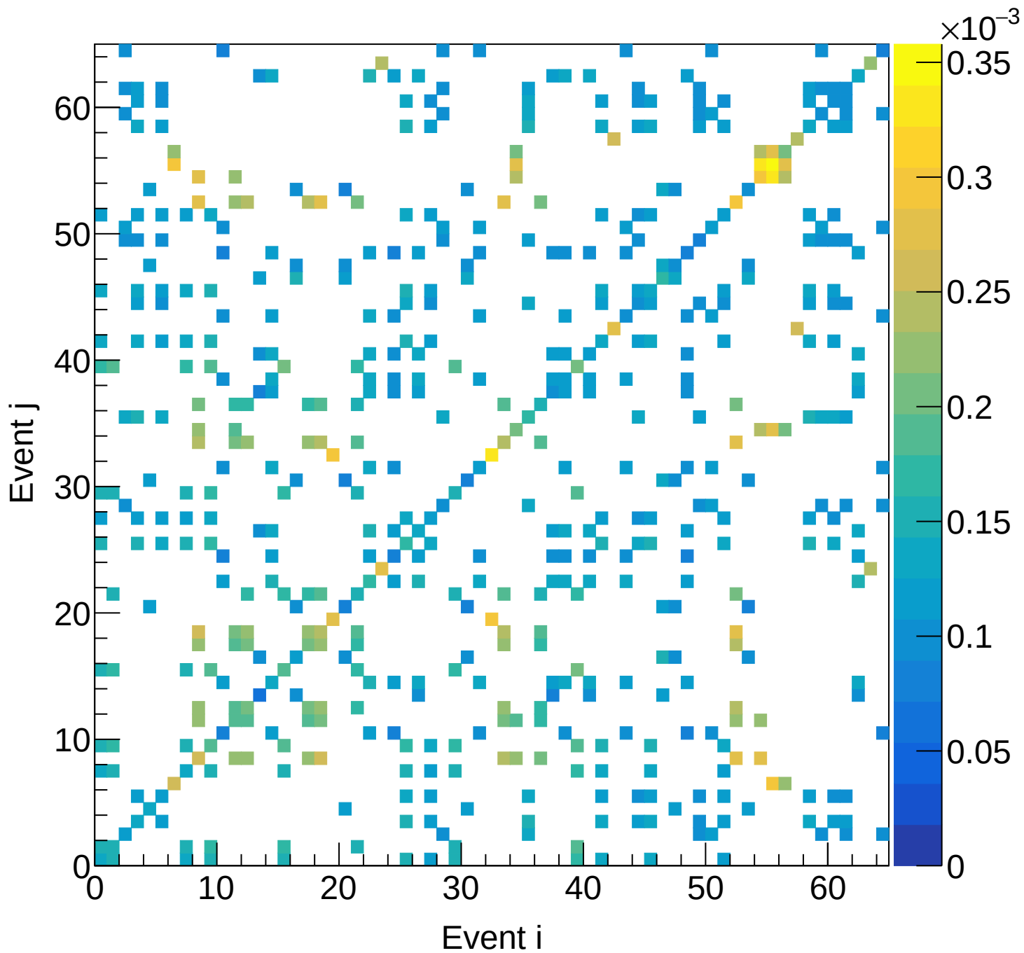
LH2 (total) Covariance | M: [5.4, 5.7) xF: [0.00, 0.05)
