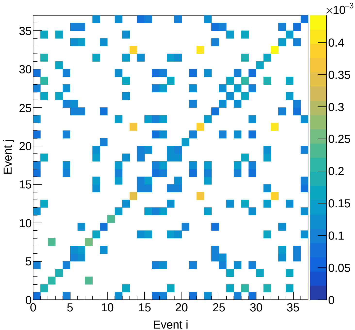
LH2 (total) Covariance | M: [5.7, 6.0] xF: [0.00, 0.05]
