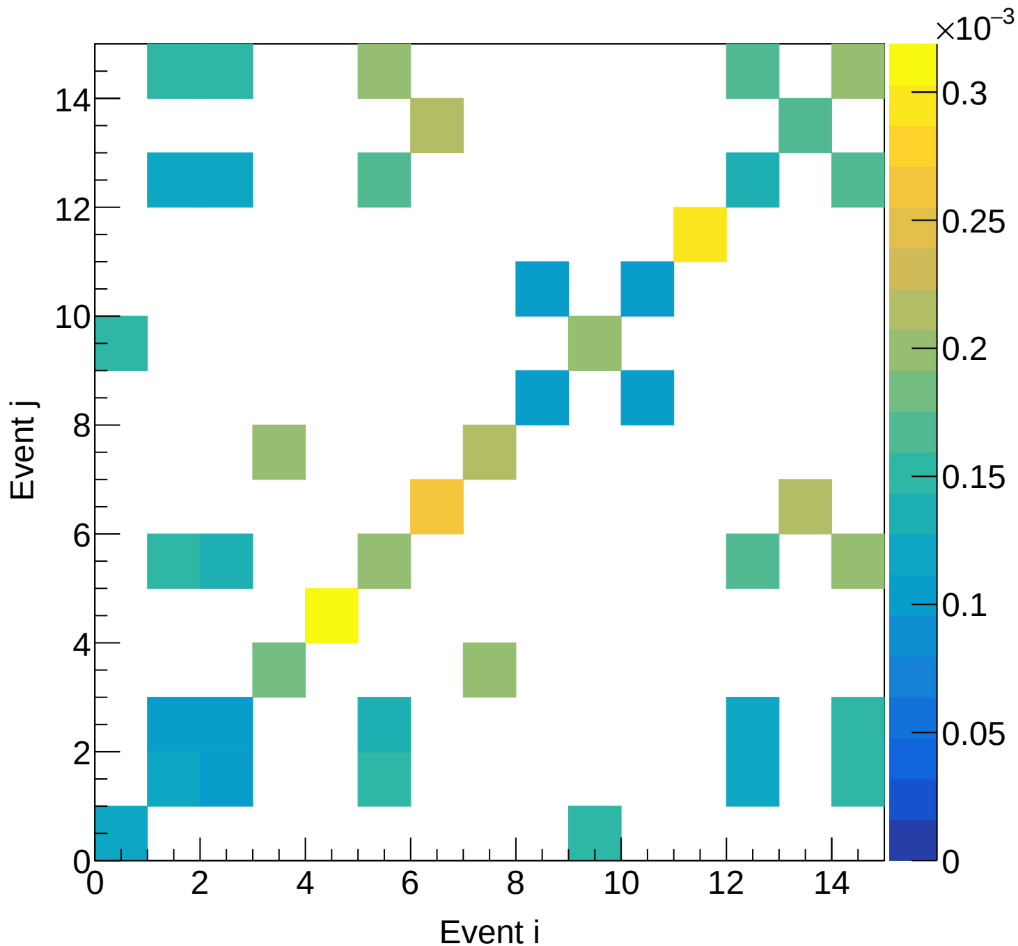
LH2 (total) Covariance | M: [6.3, 6.6) xF: [0.00, 0.05)
