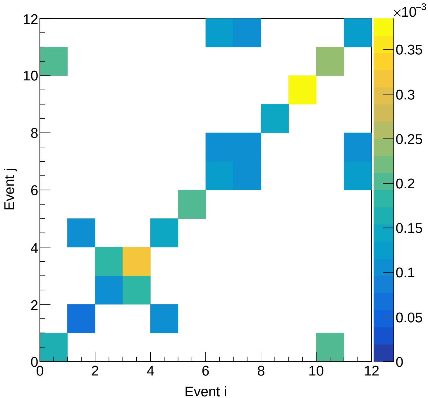
LH2 (total) Covariance | M: [6.6, 6.9) xF: [0.00, 0.05)
