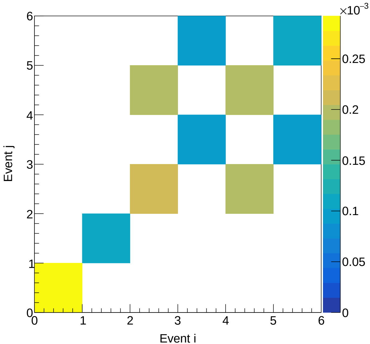
LH2 (total) Covariance | M: [7.5, 8.8) xF: [0.05, 0.10)
