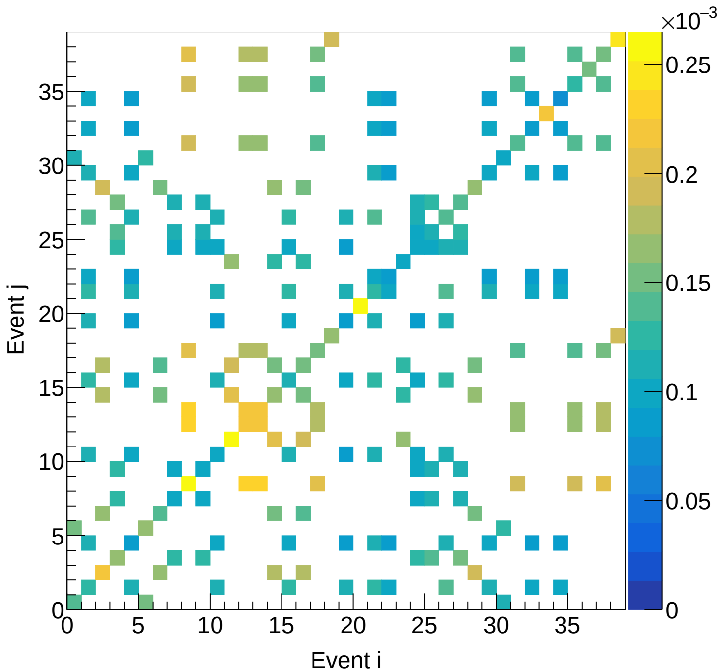
LH2 (total) Covariance | M: [6.0, 6.3) xF: [0.05, 0.10)
