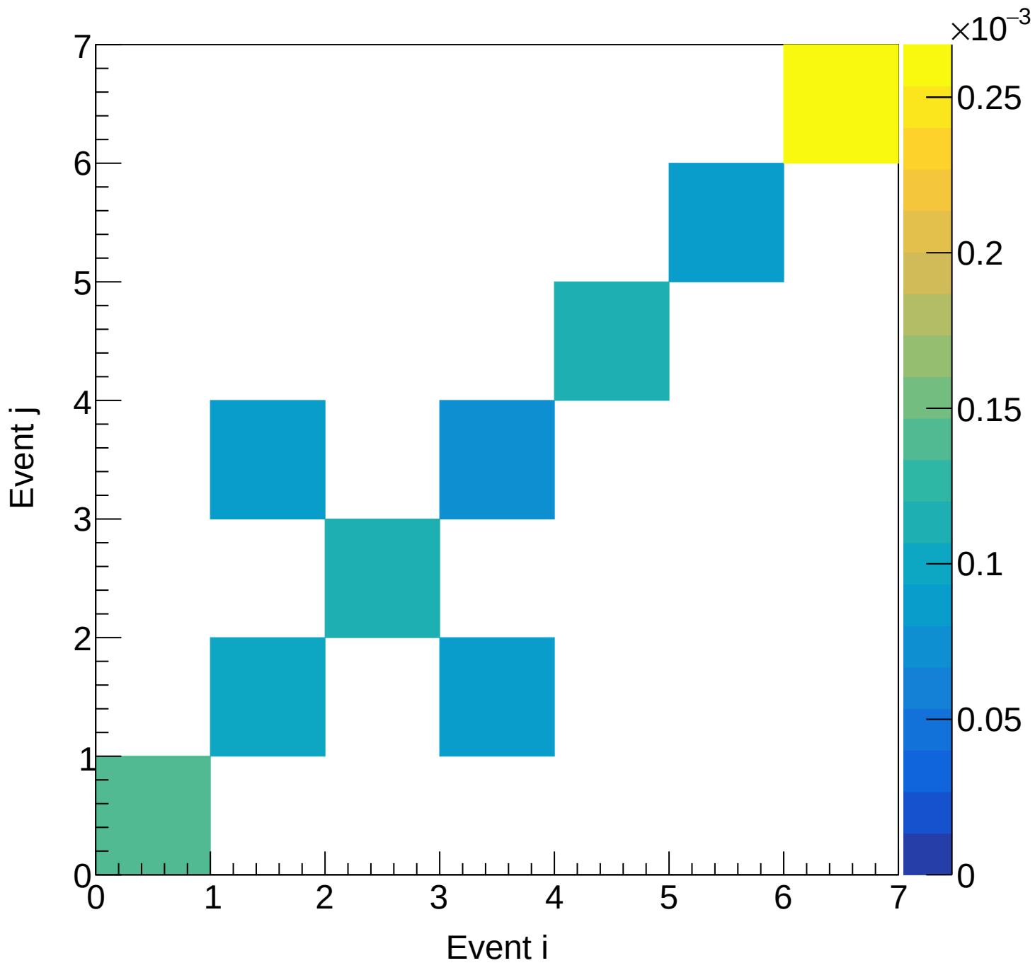
LH2 (total) Covariance | M: [7.5, 8.8) xF: [0.10, 0.15)
