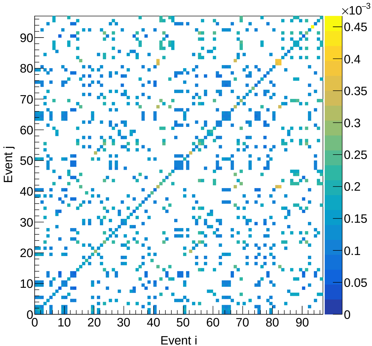
LH2 (total) Covariance | M: [4.5, 4.8) xF: [0.10, 0.15)
