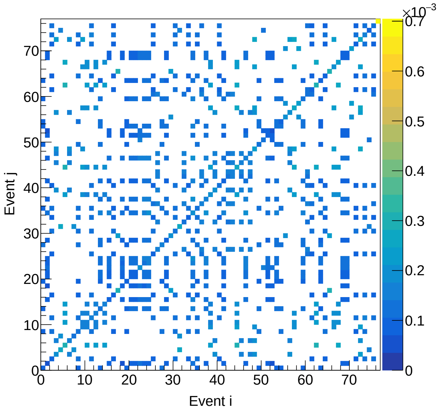
LH2 (total) Covariance | M: [5.7, 6.0] xF: [0.10, 0.15)
