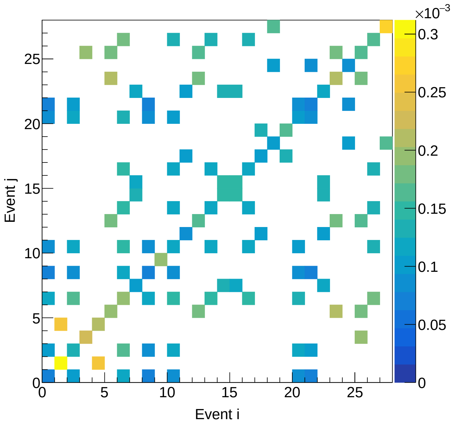
LH2 (total) Covariance | M: [6.3, 6.6] xF: [0.10, 0.15]
