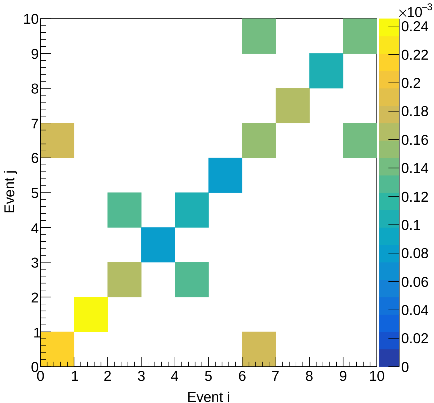
LH2 (total) Covariance | M: [6.6, 6.9) xF: [0.10, 0.15)
