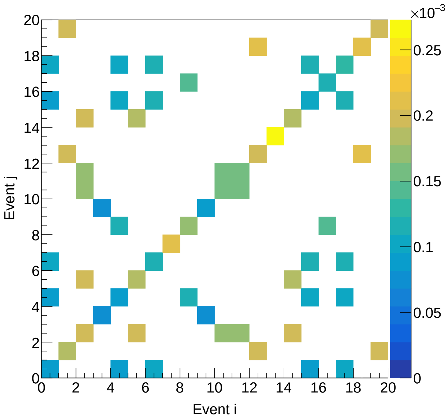
LH2 (total) Covariance | M: [3.9, 4.2) xF: [0.15, 0.20)
