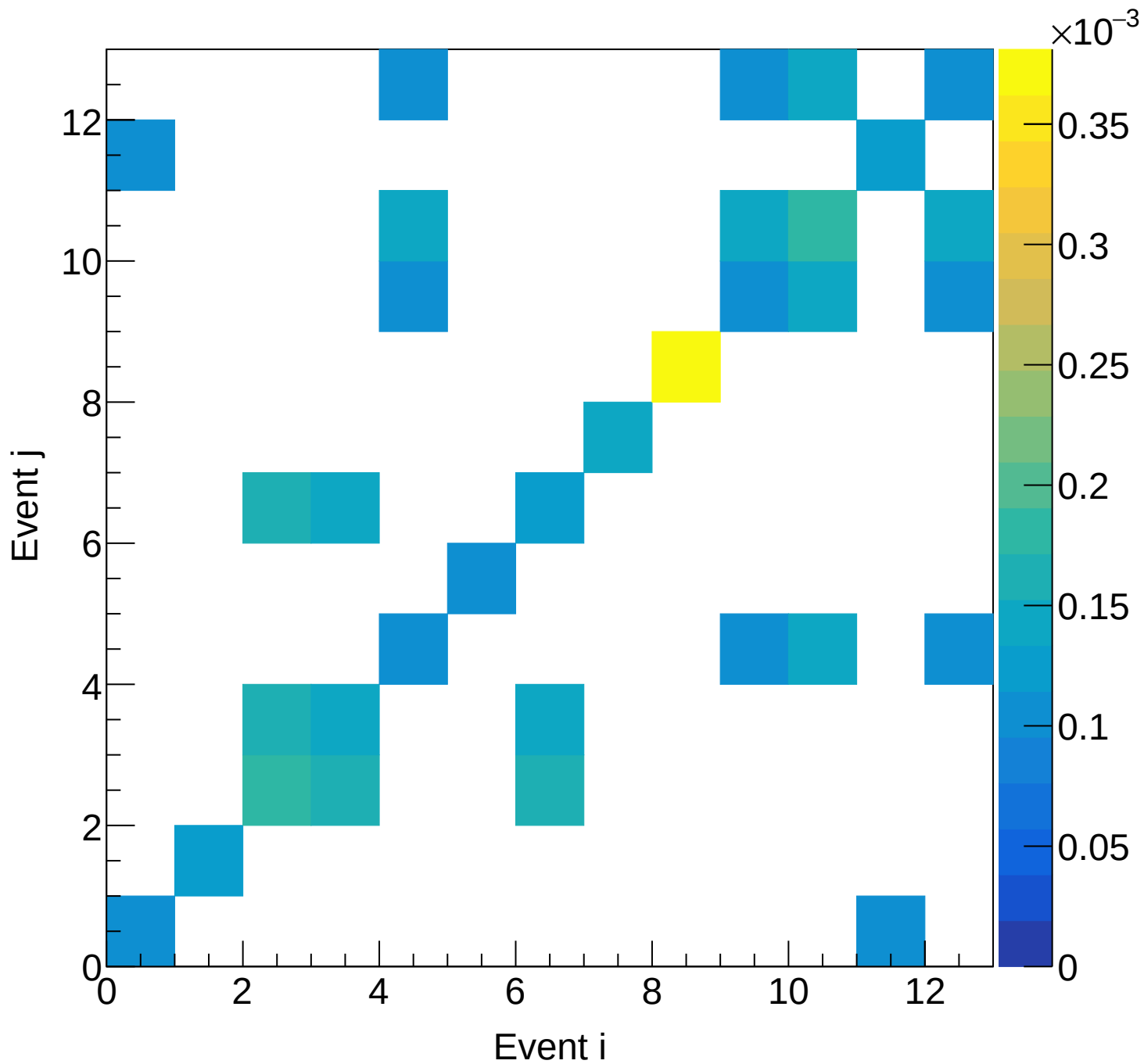
LH2 (total) Covariance | M: [6.9, 7.5) xF: [0.15, 0.20)
