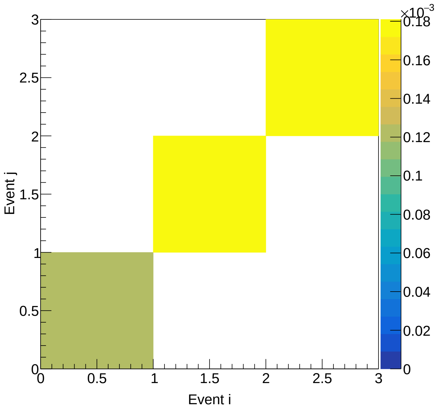
LH2 (total) Covariance | M: [7.5, 8.8) xF: [0.15, 0.20)
