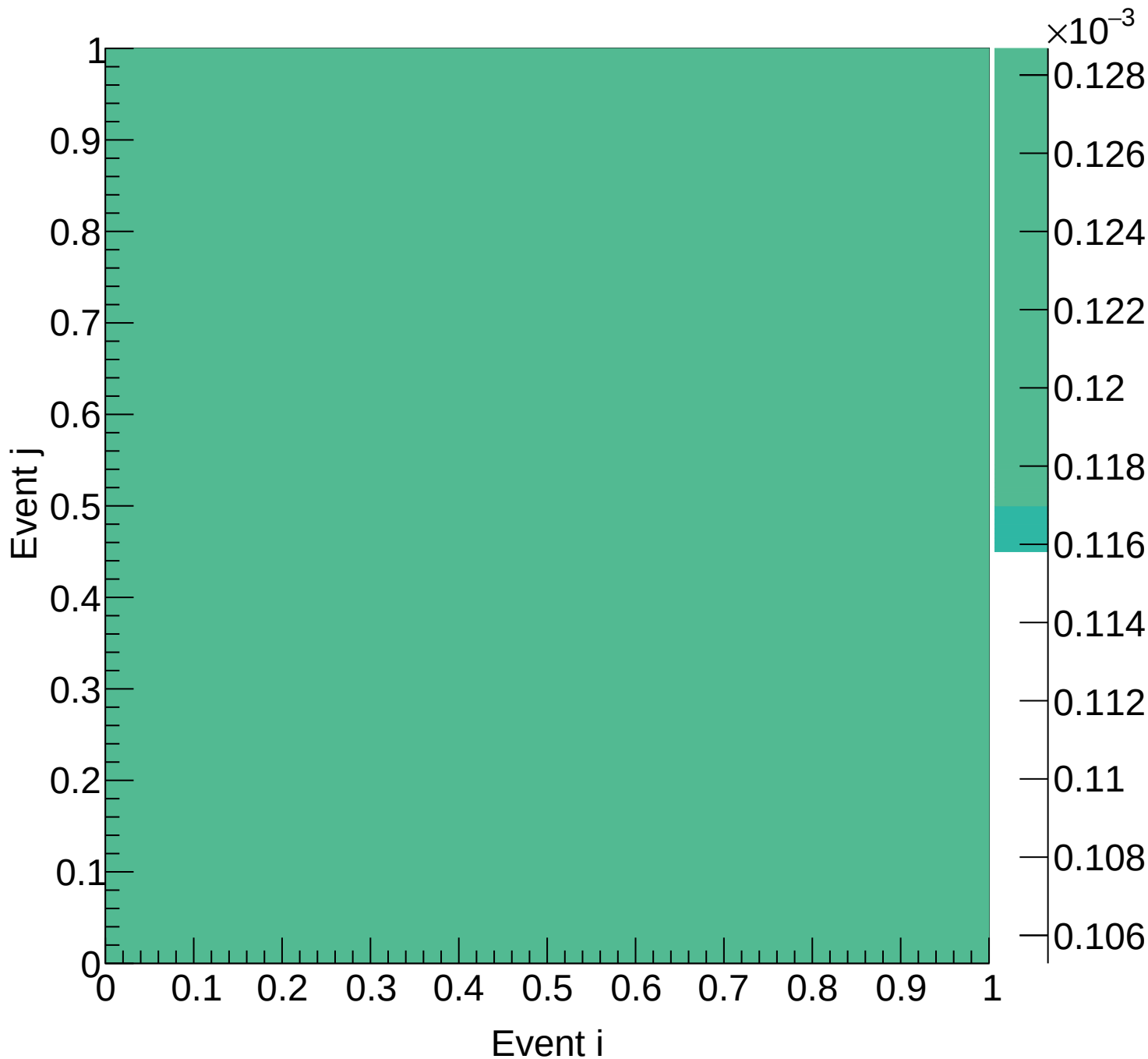
LH2 (total) Covariance | M: [8.8, 10.0) xF: [0.15, 0.20)
