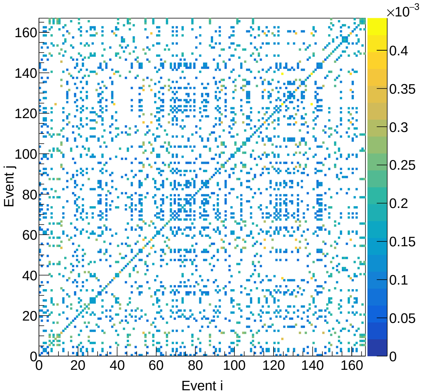
LH2 (total) Covariance | M: [4.5, 4.8) xF: [0.15, 0.20)
