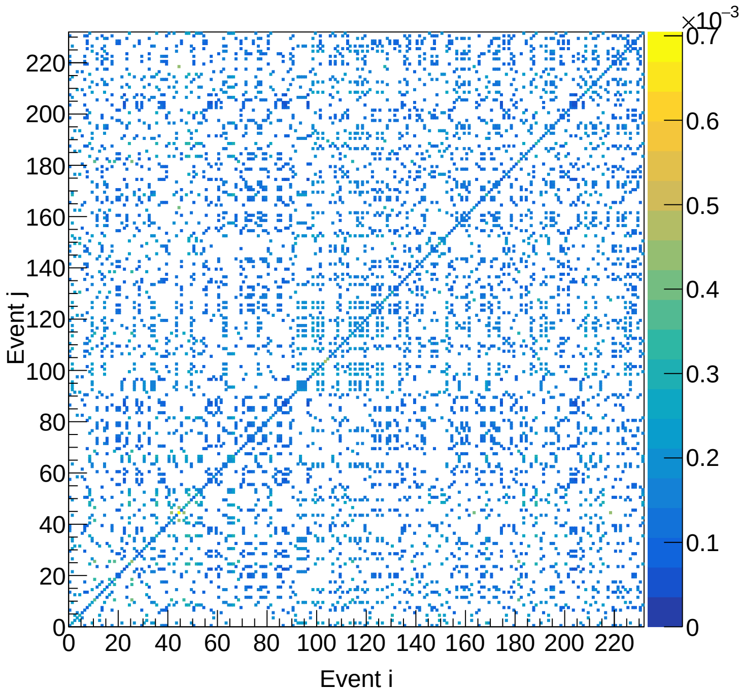
LH2 (total) Covariance | M: [4.8, 5.1) xF: [0.15, 0.20)
