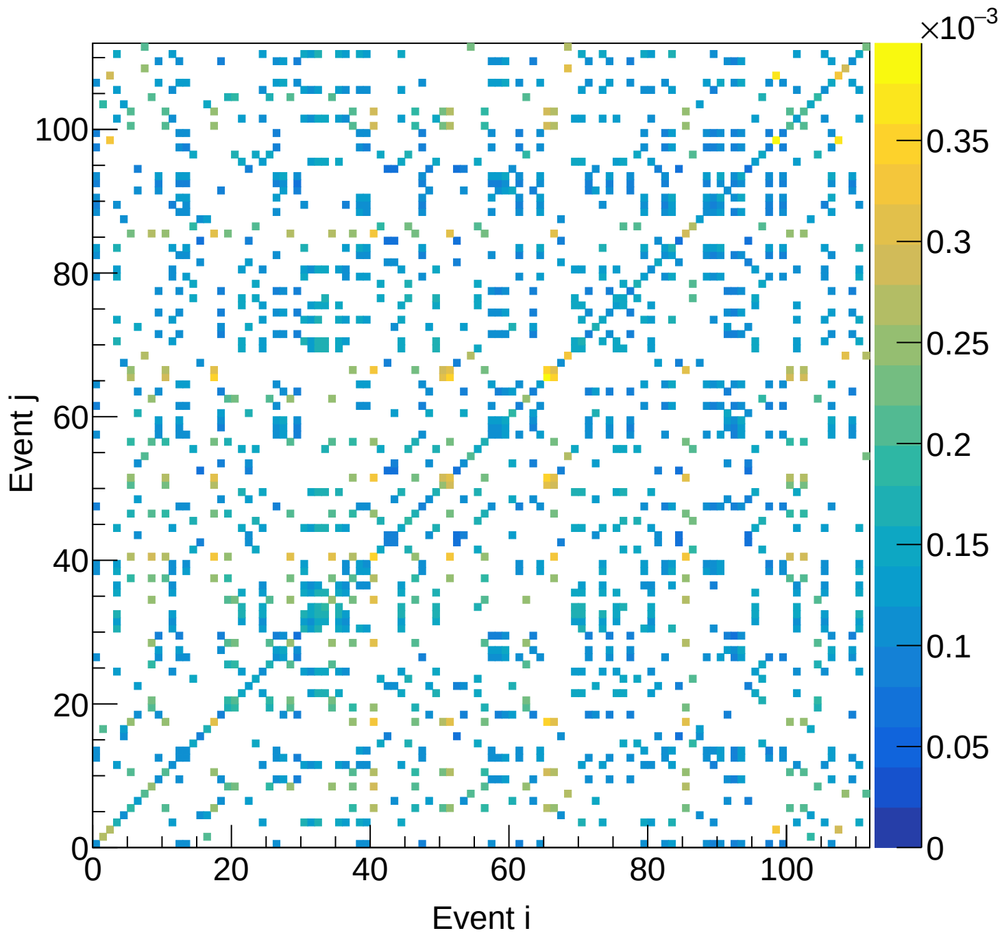
LH2 (total) Covariance | M: [5.4, 5.7) xF: [0.15, 0.20)
