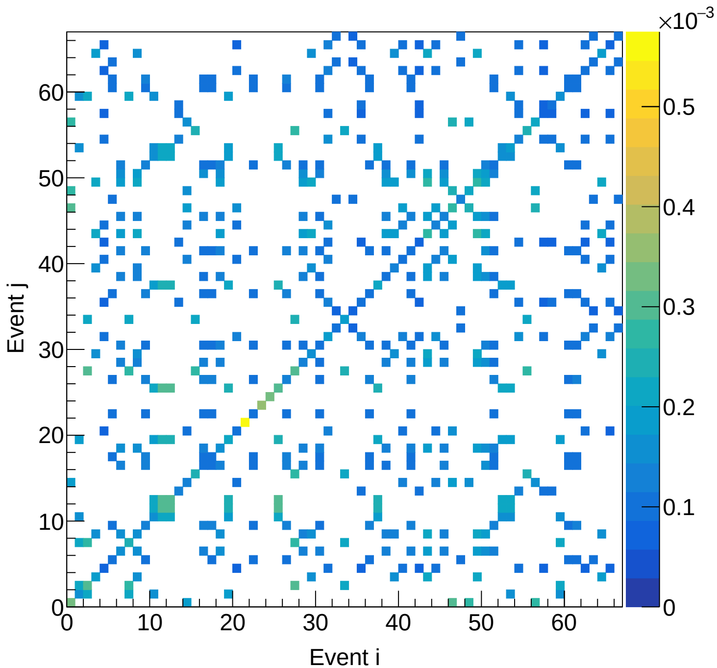
LH2 (total) Covariance | M: [6.0, 6.3) xF: [0.15, 0.20)
