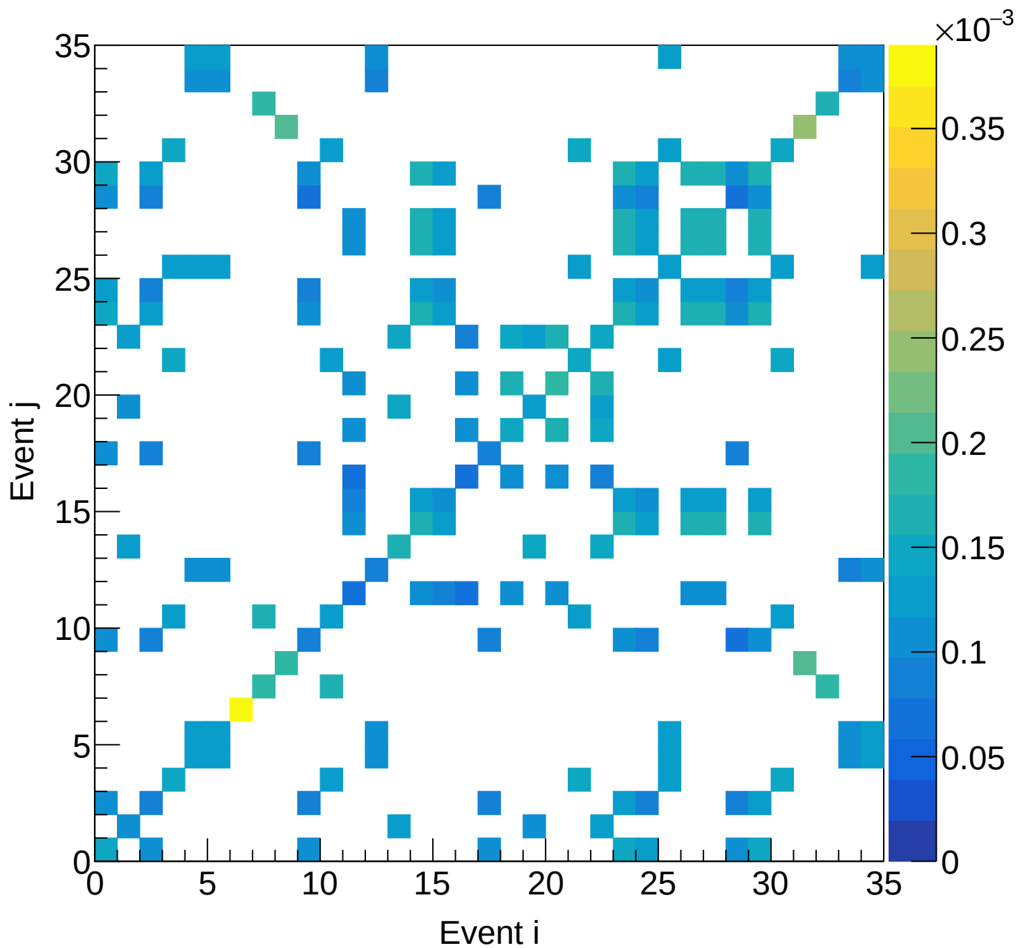
LH2 (total) Covariance | M: [6.3, 6.6) xF: [0.15, 0.20)
