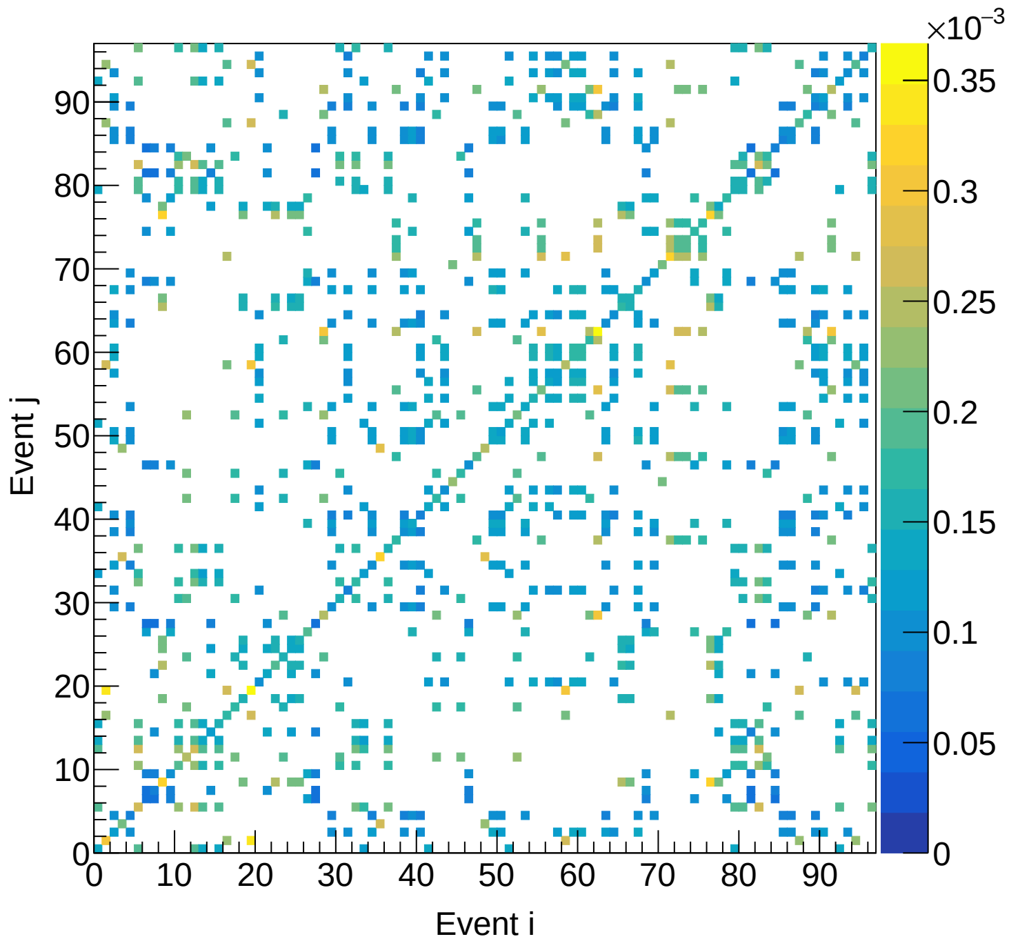
LH2 (total) Covariance | M: [3.9, 4.2) xF: [0.20, 0.25)
