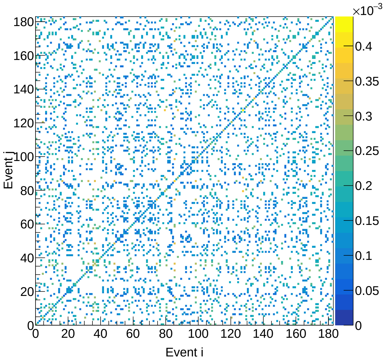
LH2 (total) Covariance | M: [4.2, 4.5) xF: [0.20, 0.25)
