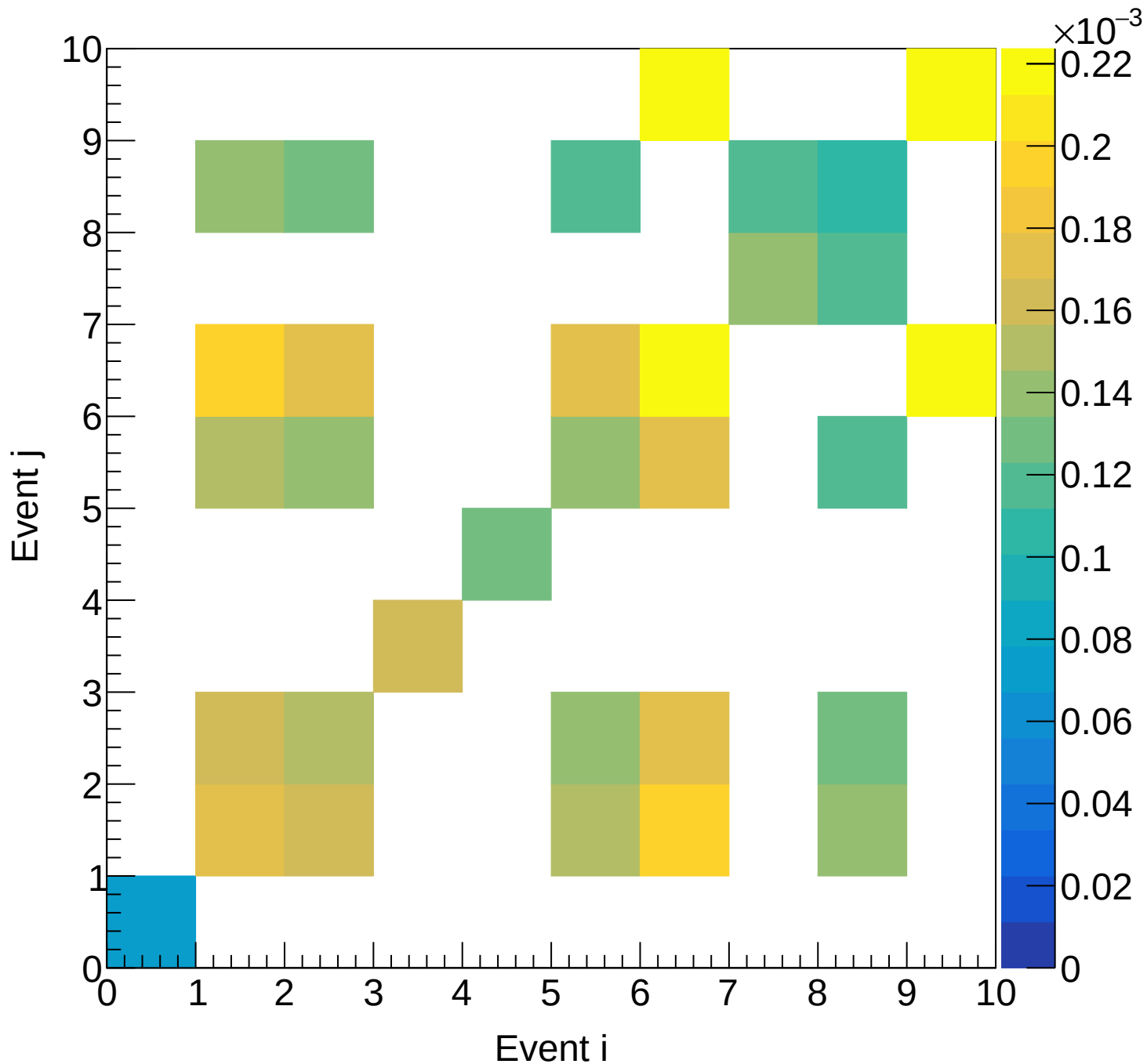
LH2 (total) Covariance | M: [6.9, 7.5) xF: [0.20, 0.25)
