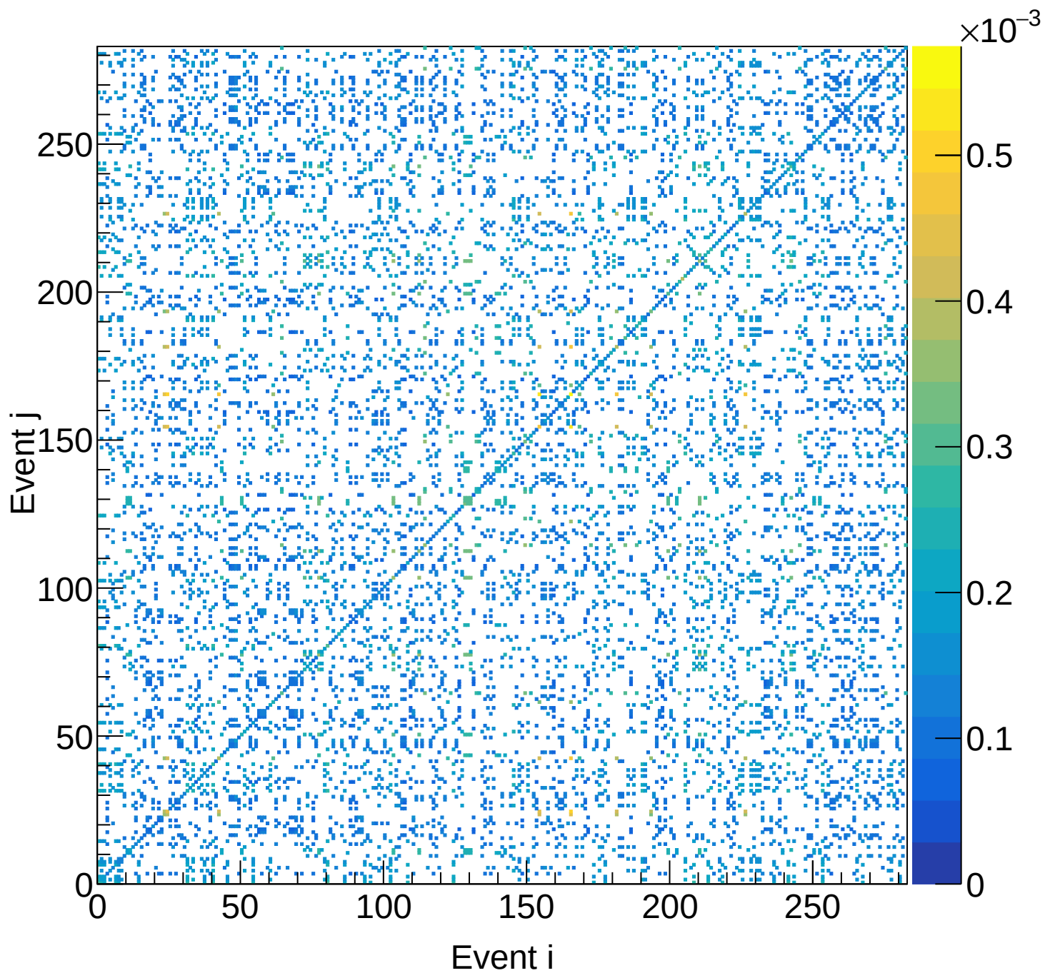
LH2 (total) Covariance | M: [4.5, 4.8) xF: [0.20, 0.25)
