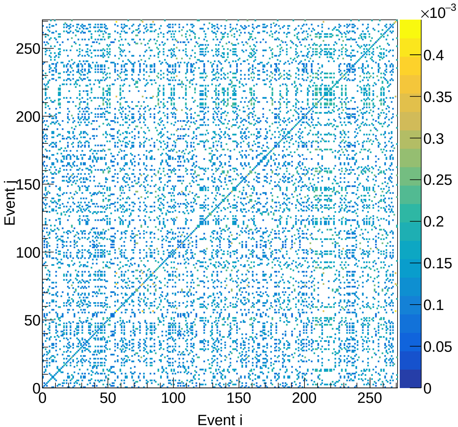
LH2 (total) Covariance | M: [4.8, 5.1) xF: [0.20, 0.25)
