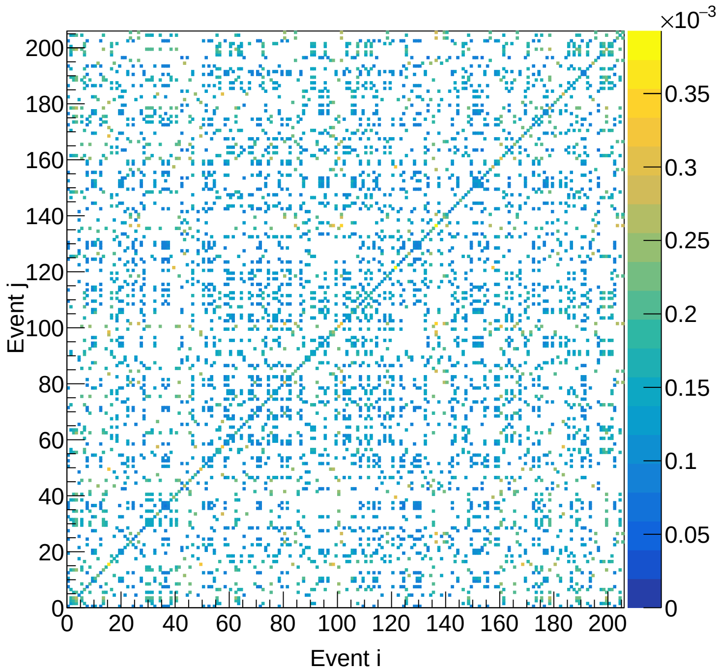
LH2 (total) Covariance | M: [5.1, 5.4) xF: [0.20, 0.25)
