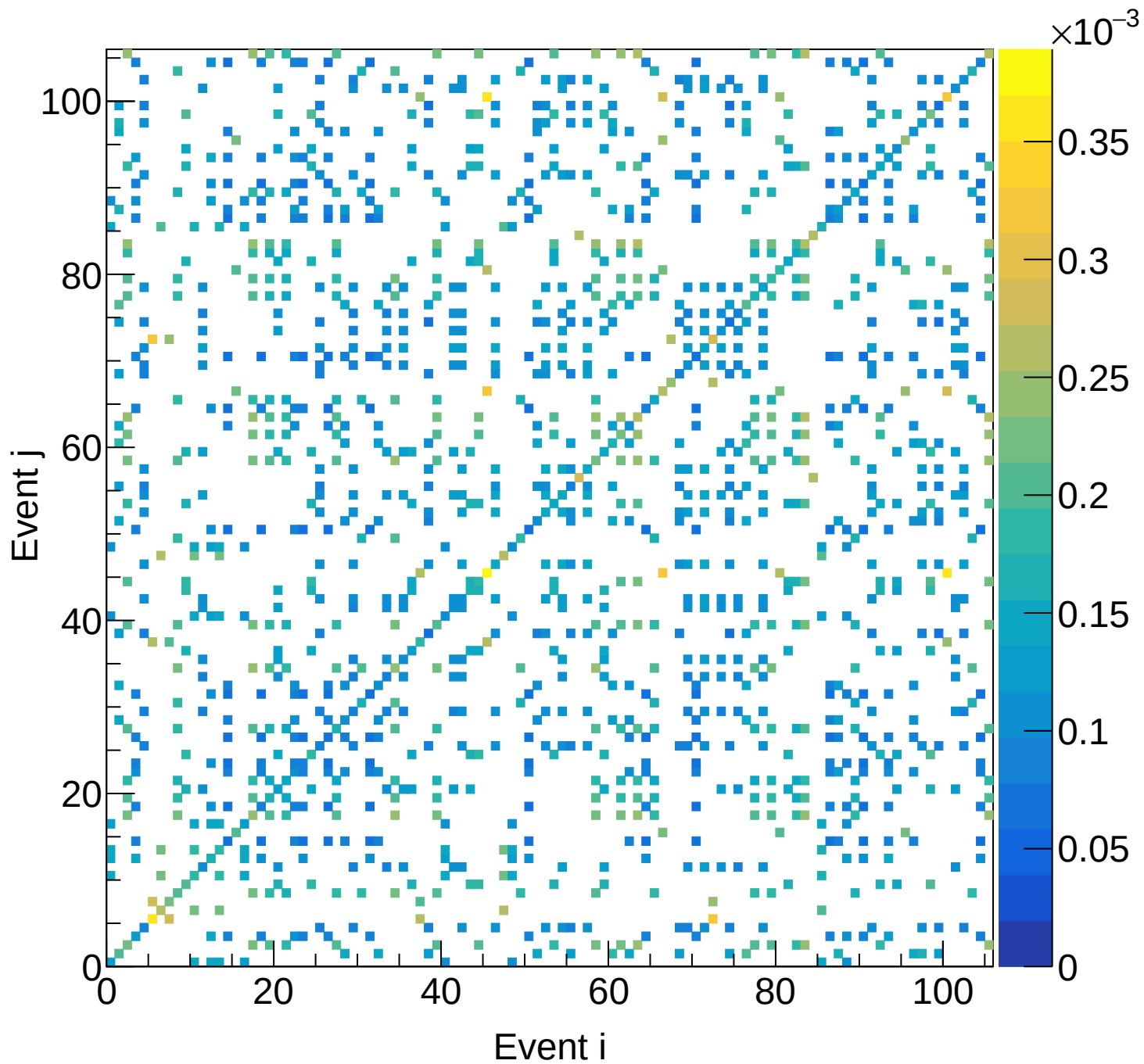
LH2 (total) Covariance | M: [5.7, 6.0] xF: [0.20, 0.25)
