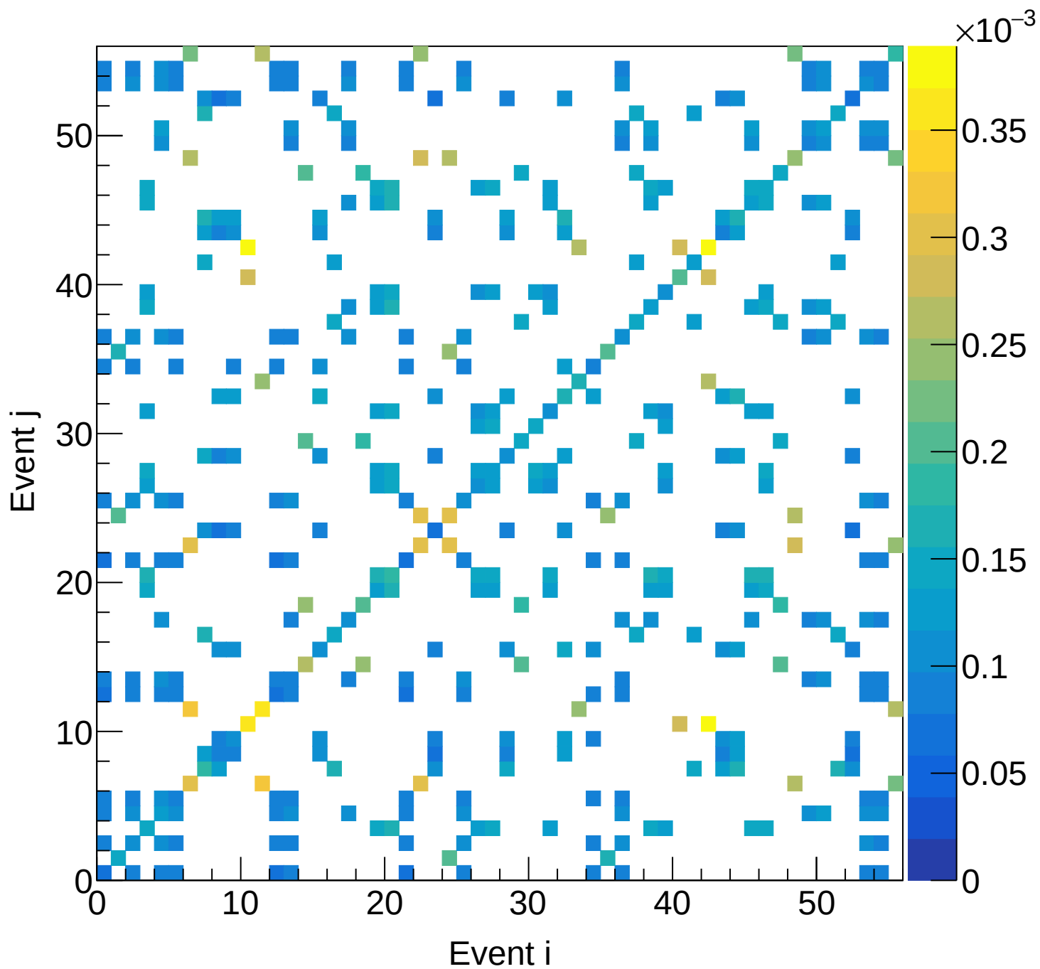
LH2 (total) Covariance | M: [6.0, 6.3) xF: [0.20, 0.25)
