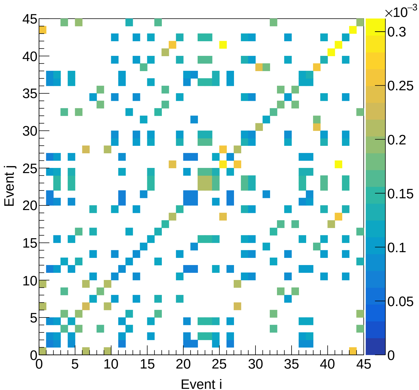
LH2 (total) Covariance | M: [6.3, 6.6) xF: [0.20, 0.25)
