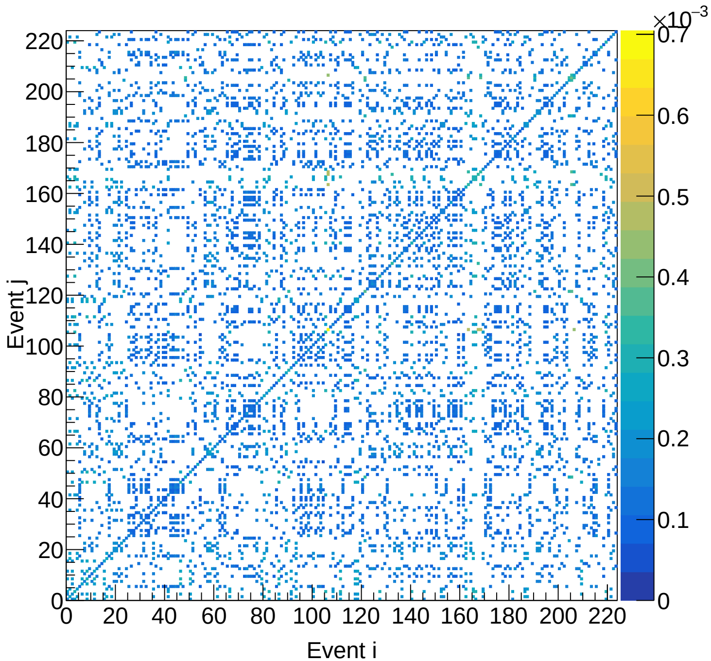
LH2 (total) Covariance | M: [3.9, 4.2) xF: [0.25, 0.30)
