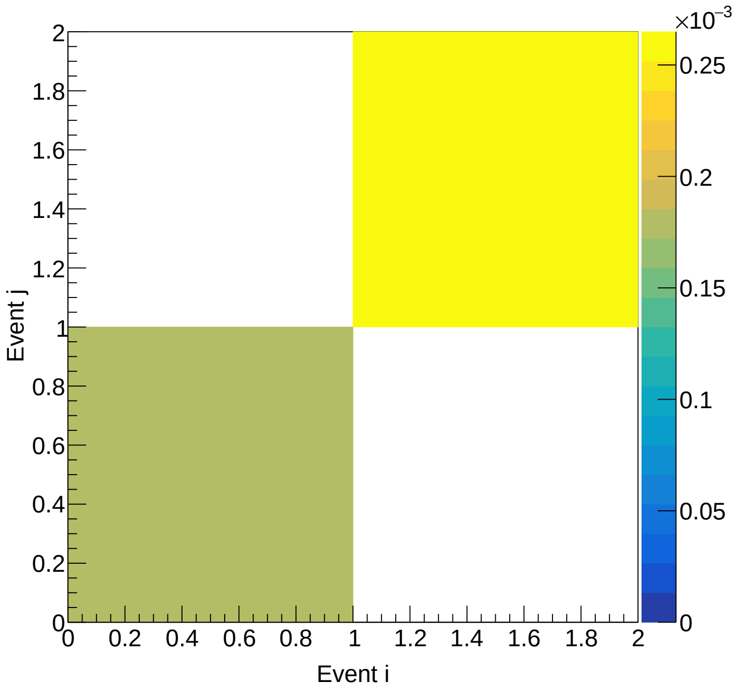
LH2 (total) Covariance | M: [7.5, 8.8) xF: [0.25, 0.30)
