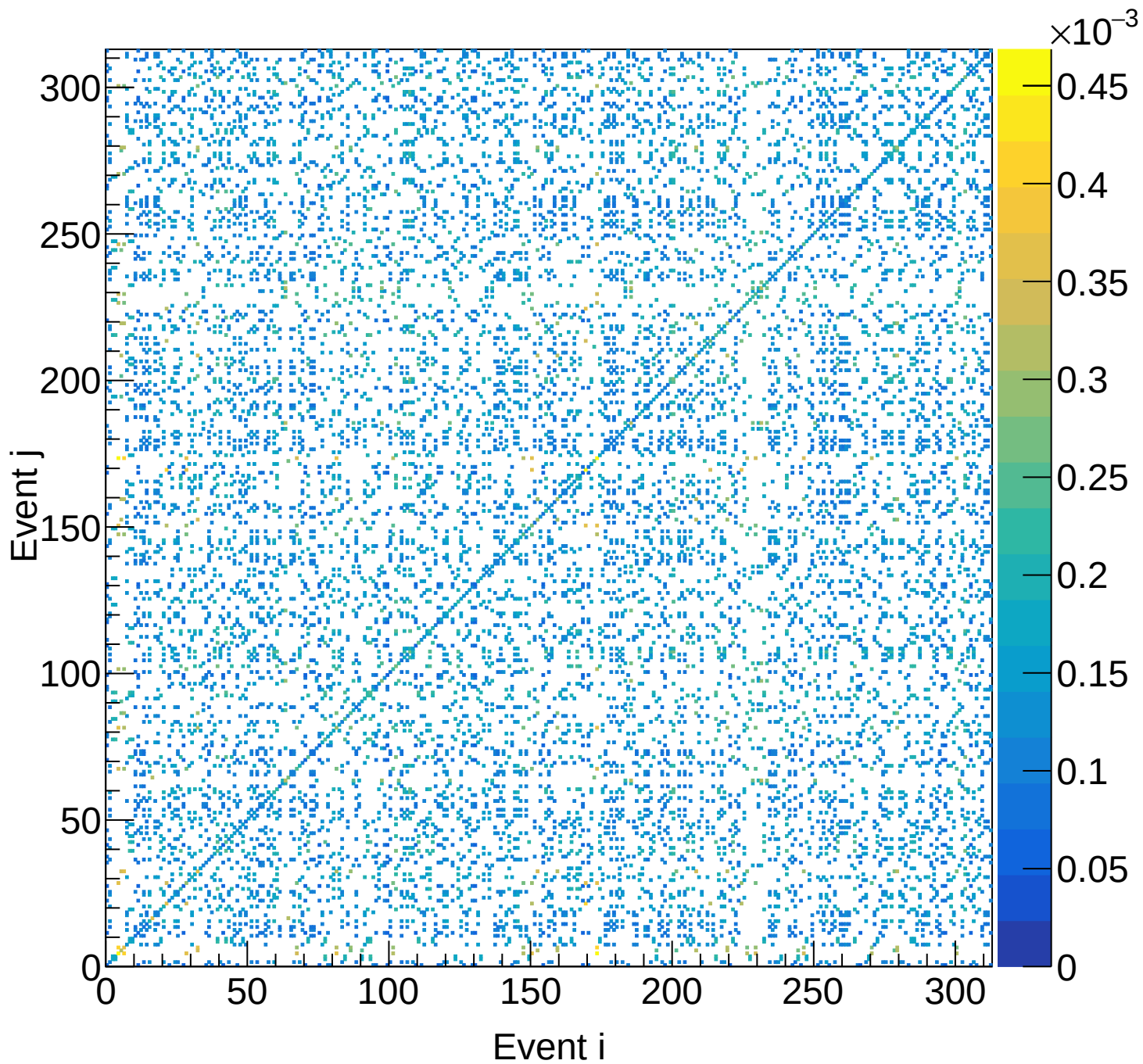
LH2 (total) Covariance | M: [4.8, 5.1) xF: [0.25, 0.30)
